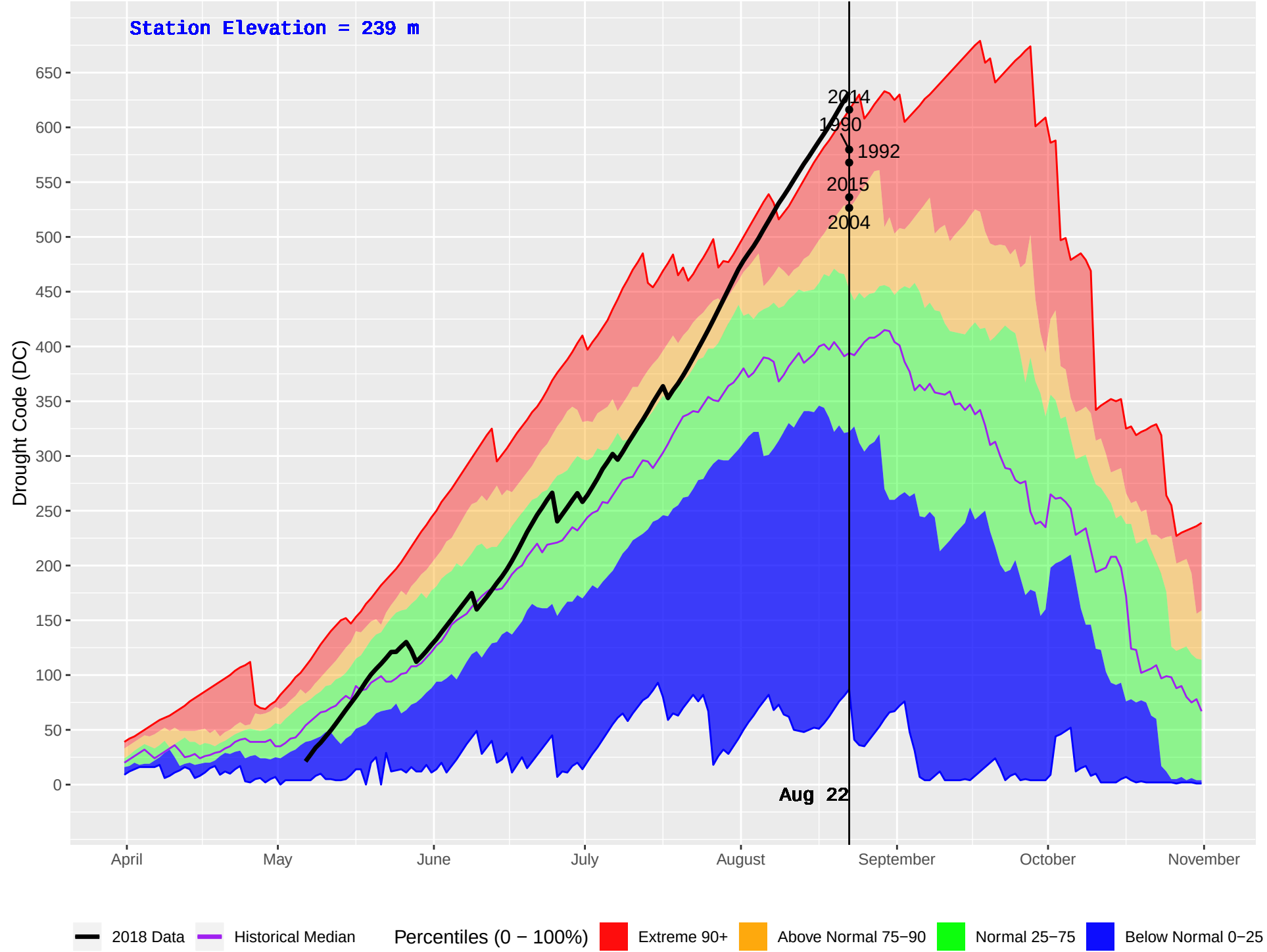
ROSSWOOD (105) : Historical (1970–2016) and Current (2018) Daily Drought Code (DC)
