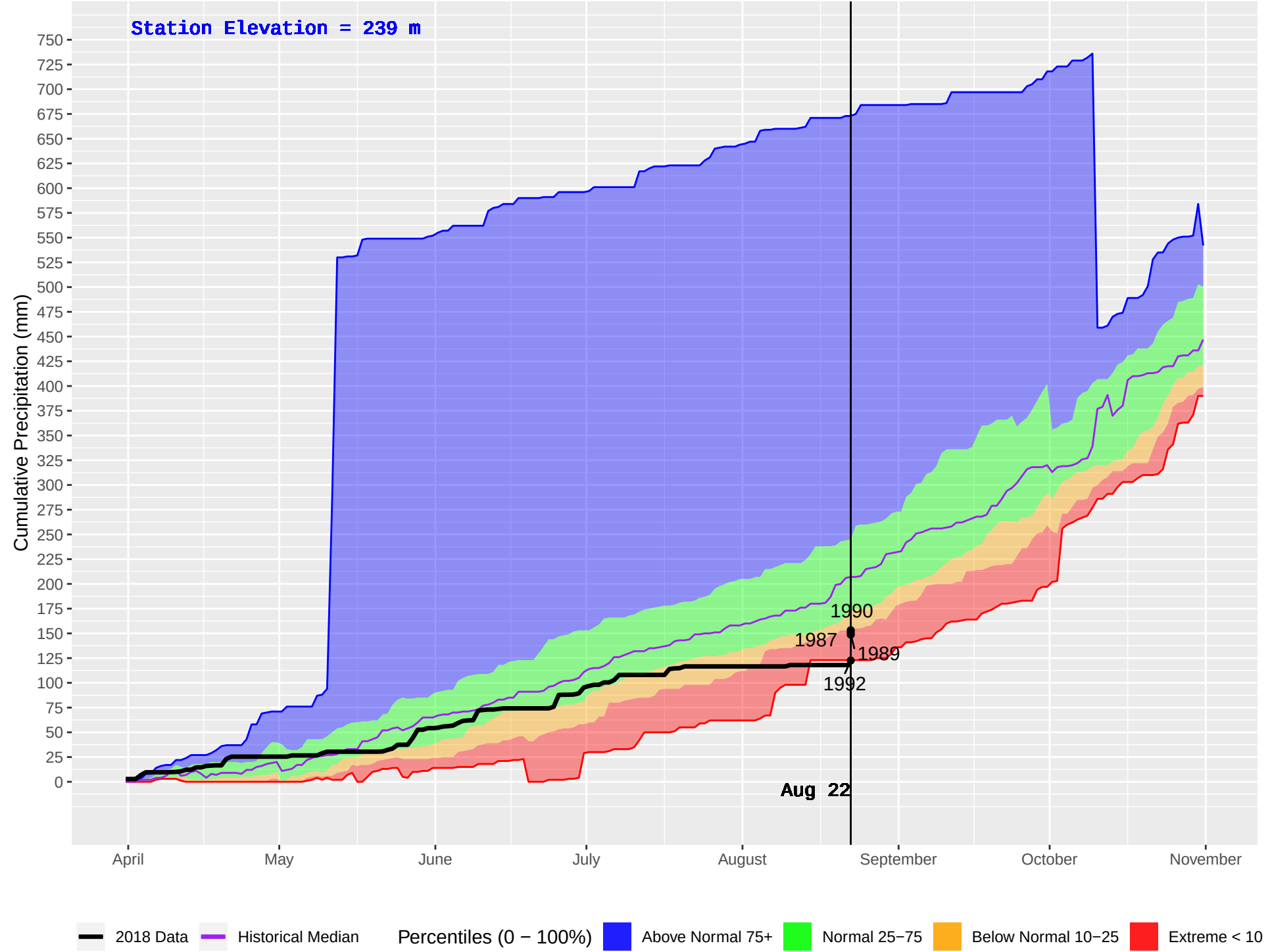
ROSSWOOD (105) : Historical (1970–2016) and Current (2018) Daily Cumulative Precipitation
