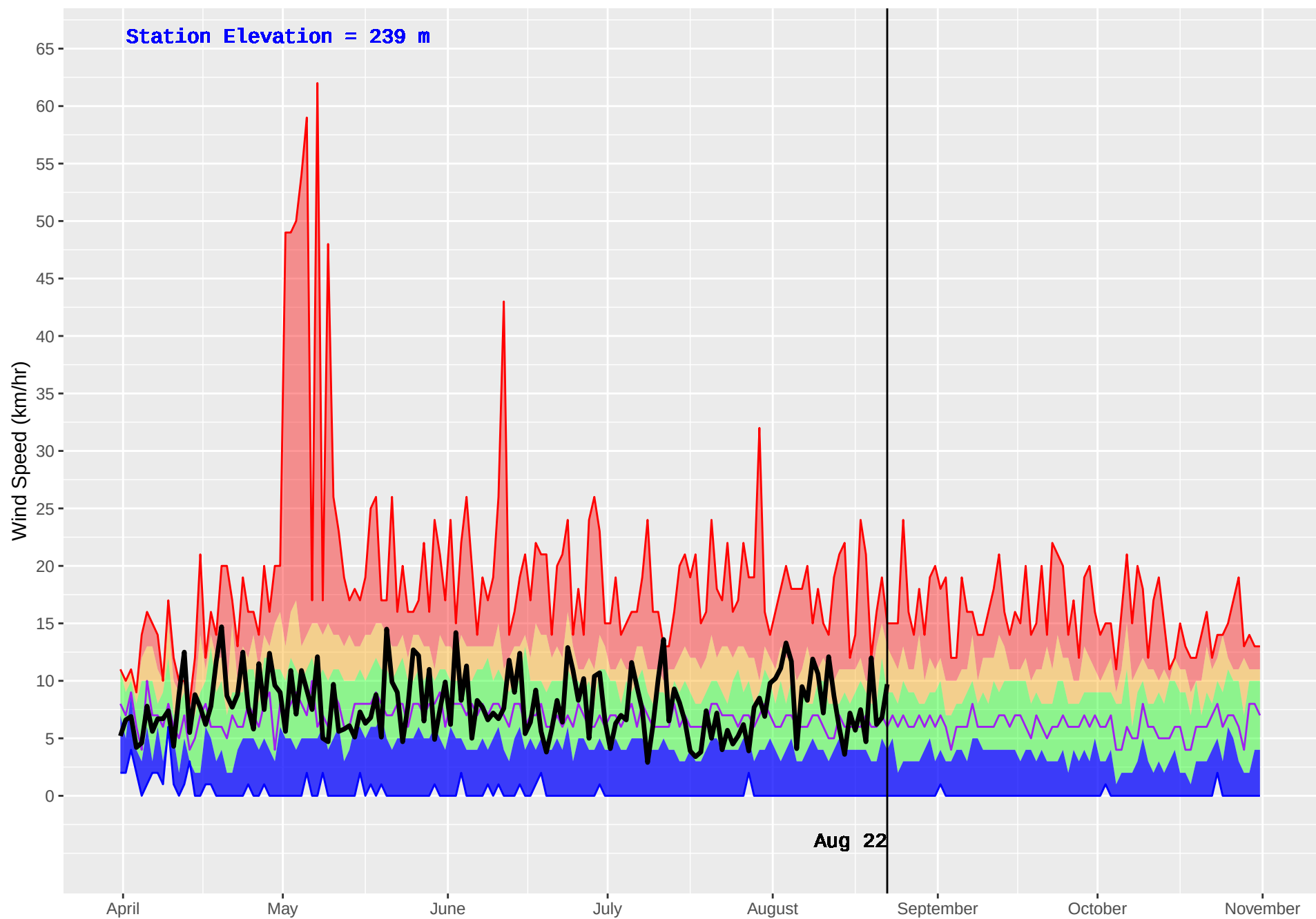
ROSSWOOD (105) : Historical (1970–2016) and Current (2018) Daily Wind Speed
