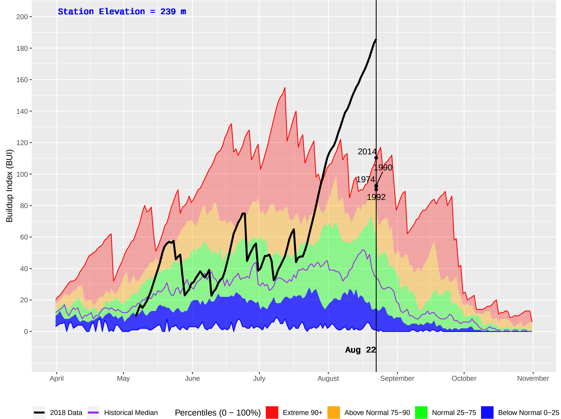
ROSSWOOD (105) : Historical (1970–2016) and Current (2018) Daily Buildup Index (BUI)
