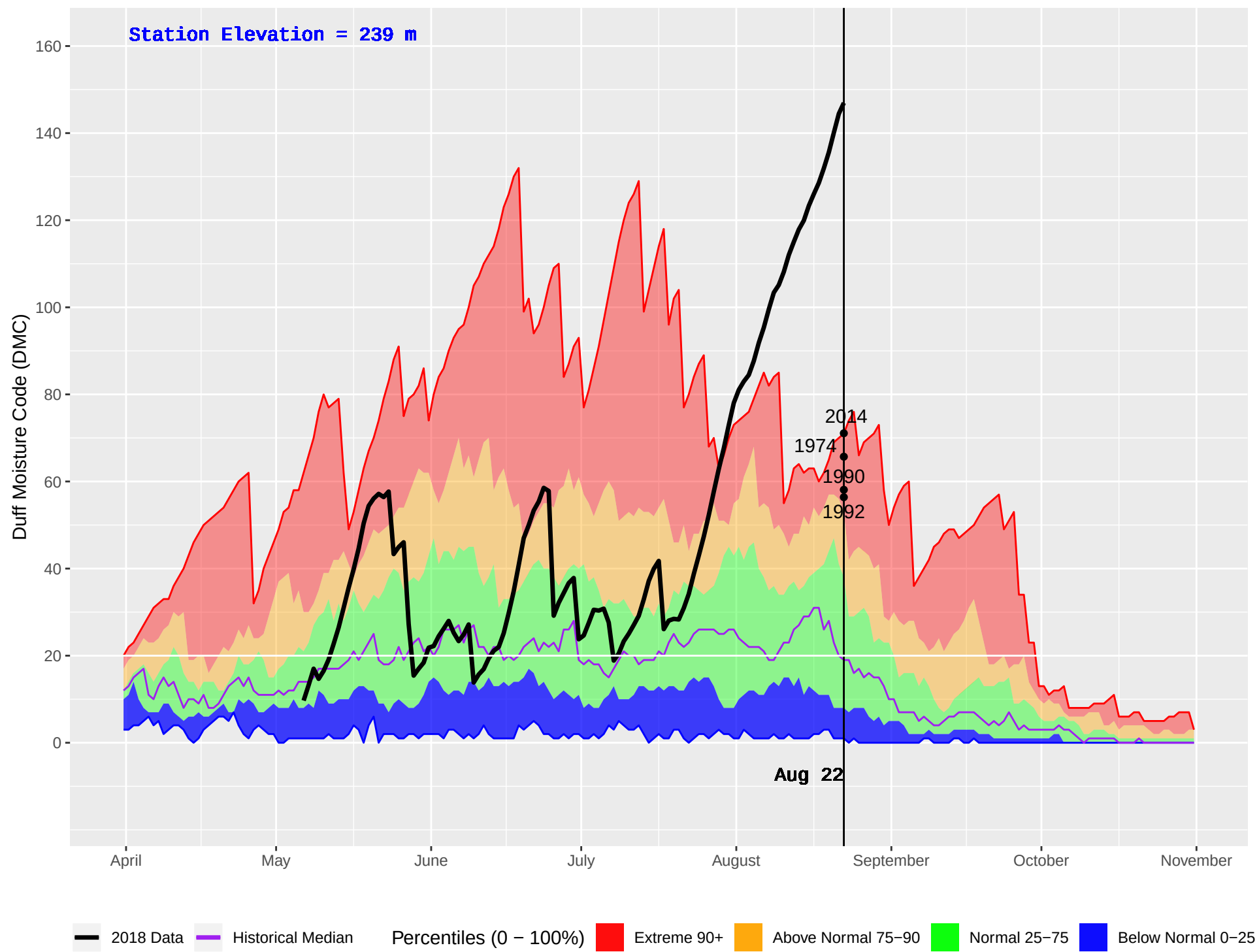
ROSSWOOD (105) : Historical (1970–2016) and Current (2018) Daily Duff Moisture Code (DMC)
