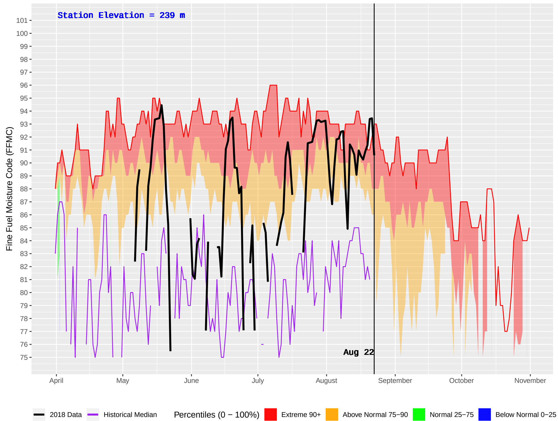
ROSSWOOD (105) : Historical (1970–2016) and Current (2018) Daily Fine Fuel Moisture Code (FFMC)
