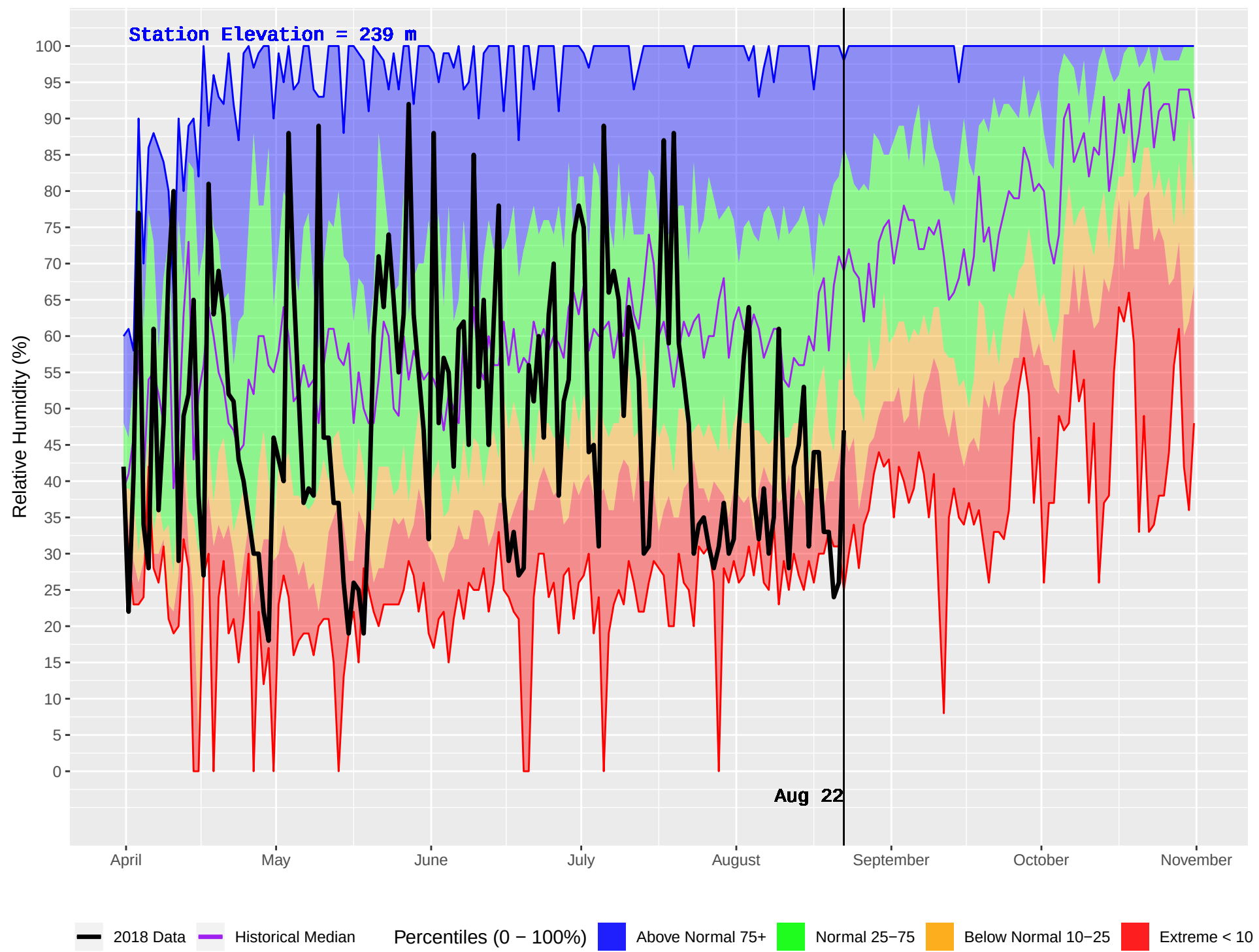
ROSSWOOD (105) : Historical (1970–2016) and Current (2018) Daily Relative Humidity
